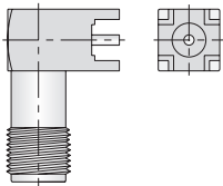
54. PCB Mt. R/A jack
